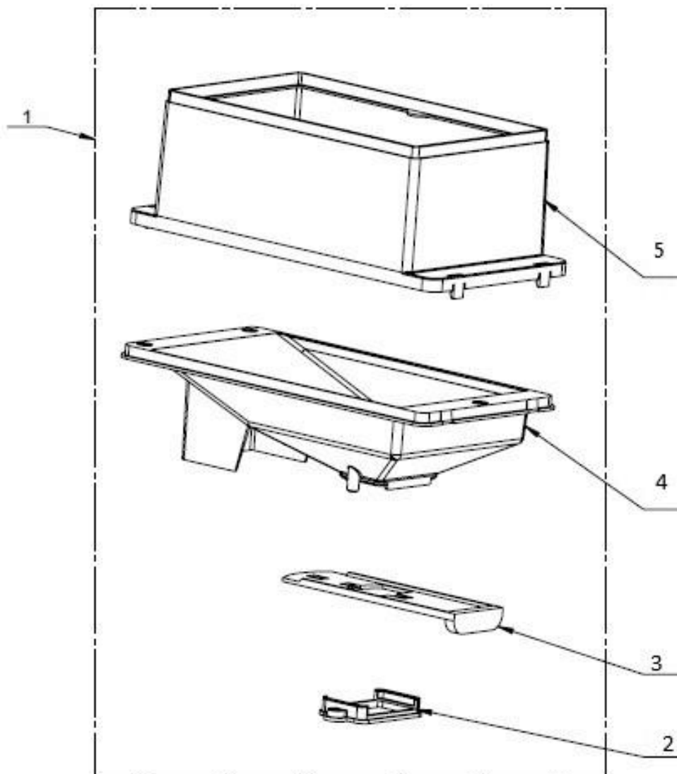
f - JL26 Coffee Bean Container Assembly
